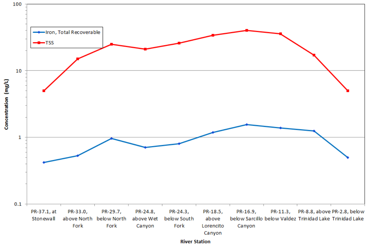
Figure 3 – Correlation Between TSS and Total Recoverable Iron in the Purgatoire – June 2014
